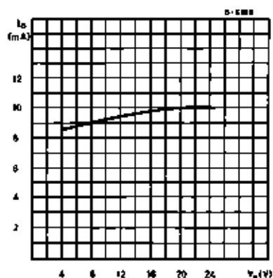
Figure 1 : Quiescent Current vs. Supply Voltage
